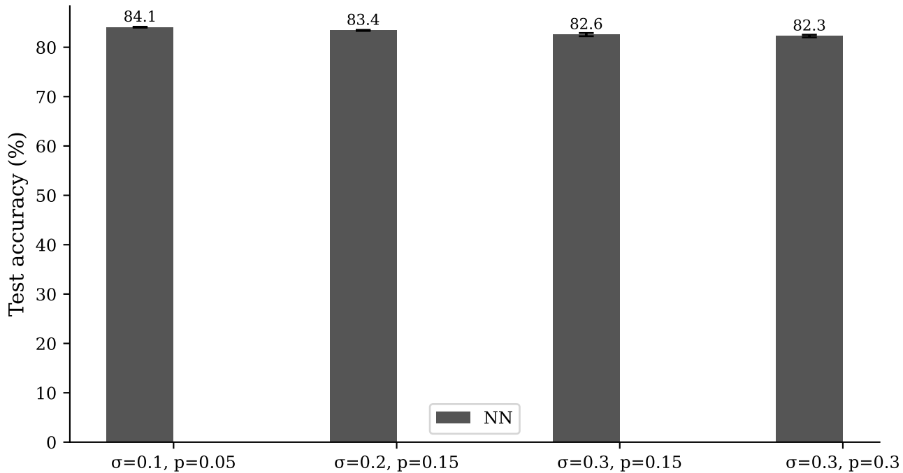
NN: combined feature + label noise
